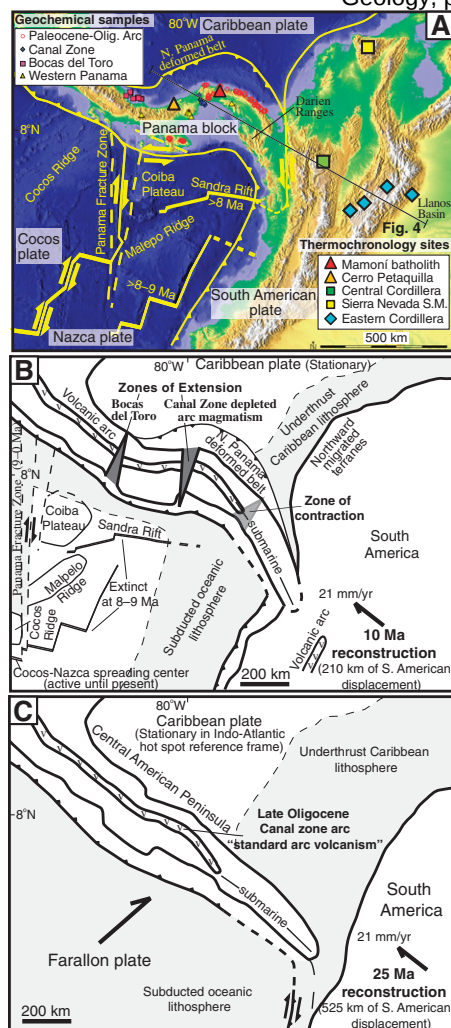
Figure 1. A: Modern tectonic map with location of geochemical samples and low-temperature thermochronology profile sites. S.M.—Santa Marta. B: Tectonic reconstruction at 10 Ma. This is an intermediate step in the collision between South America and Panama. The Panama block has fractured, resulting in two zones of extension (Canal Zone and Bocas del Toro) and one zone of contraction in eastern Panama. Also, the North Panama deformed belt has partially formed and a seaway >200 km wide separates Panama and South America. C: Tectonic reconstruction at 25 Ma. This immediately precedes collision between Panama arc crust and South America. Previously, unmodified Caribbean crust was underthrust beneath South America.
